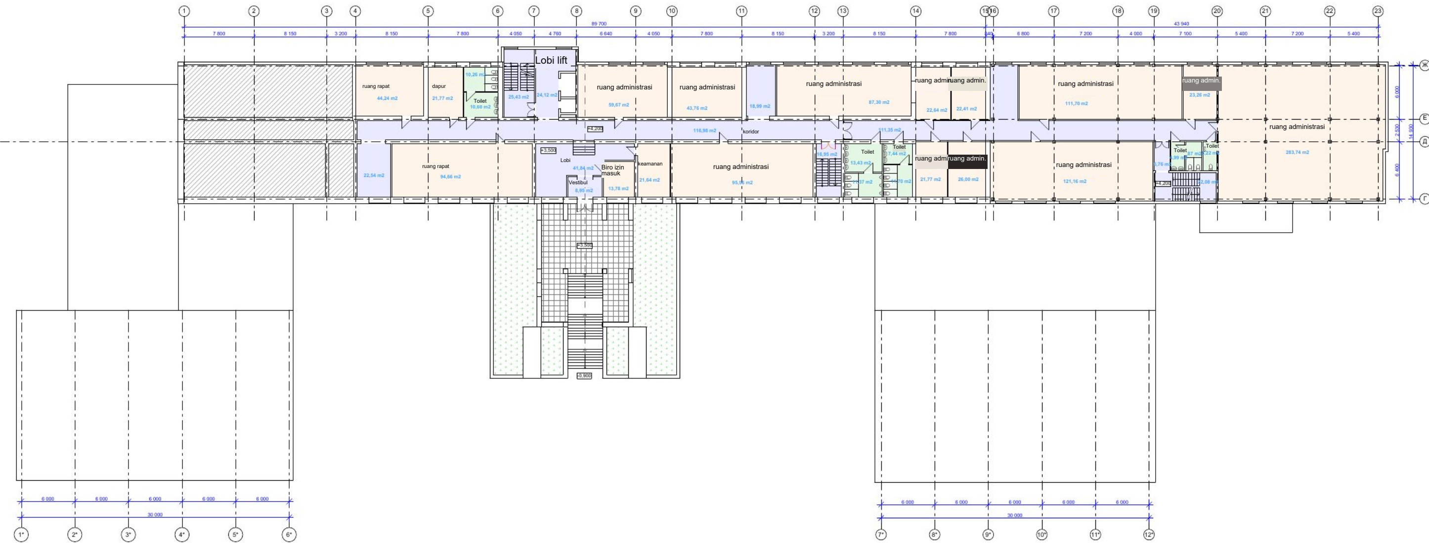
Denah lantai 2
